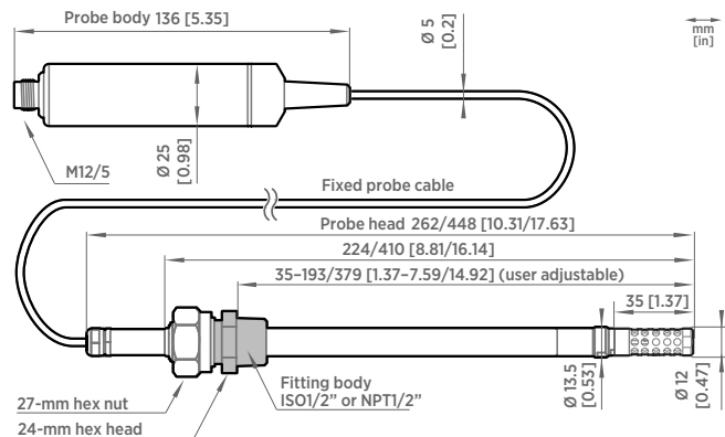
MMP8 dimensions
