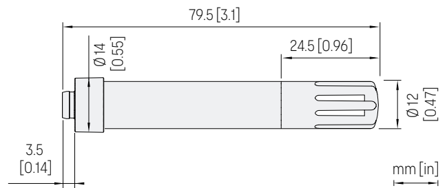
HMP113 dimensions
