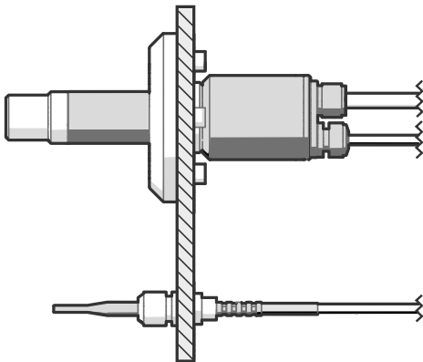
HPP272MOUNTINGSET2
