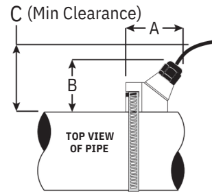
UZ Adjustable Small Pipe
