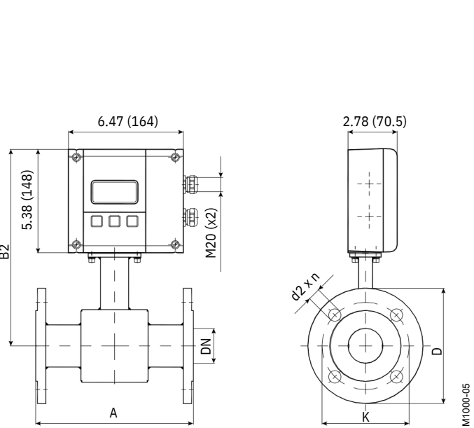
Process Connection Flange Mounted Version in. (mm)
