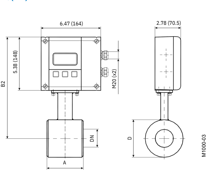
Process Connection Wafer Mounted Version in. (mm)
