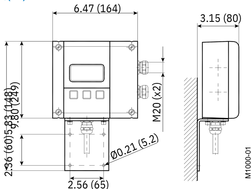
ModMAG M1000 Transmitter in. (mm)
