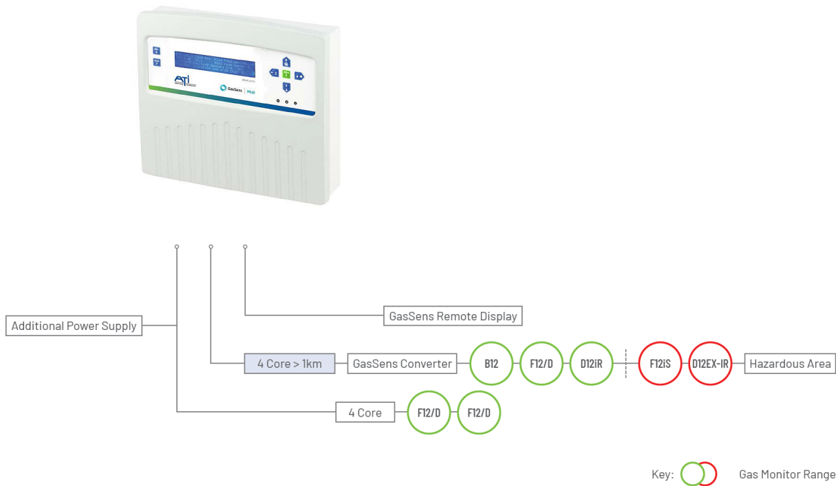
Figure 1: Sample connectivity diagram
