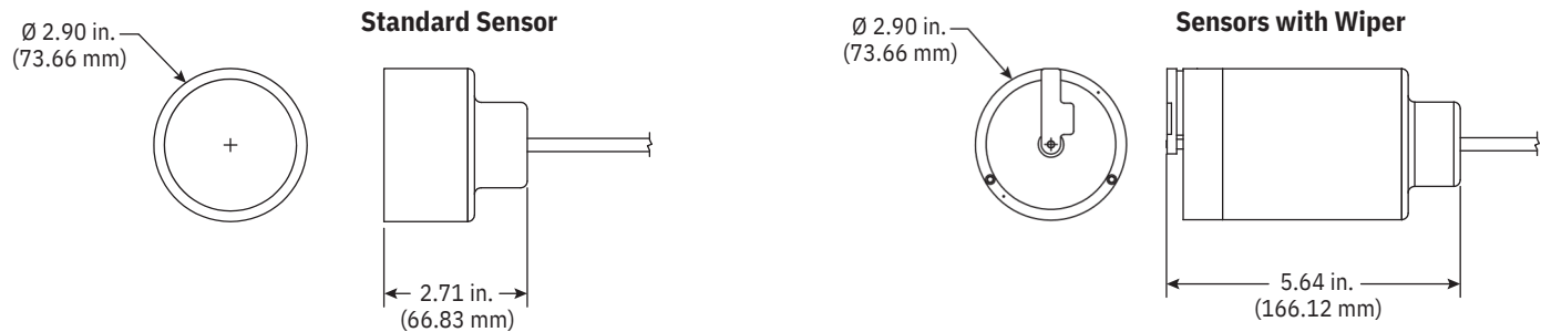
Figure 2: EchoSmart sensor dimensions
