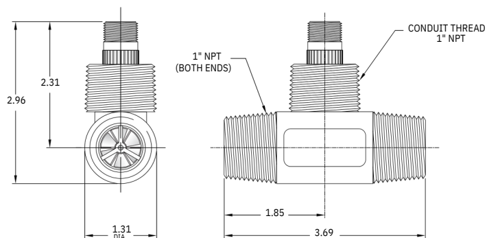
Figure 3: Dimensions
