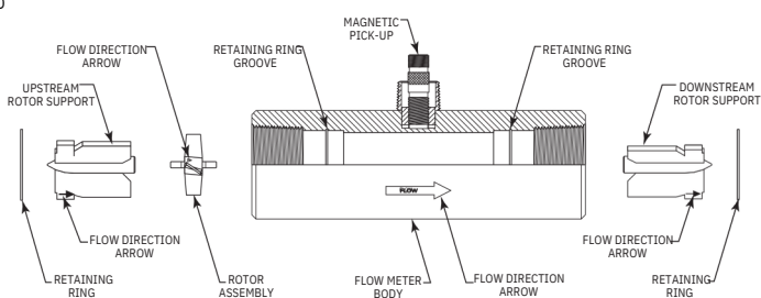
Figure 4: Exploded View
